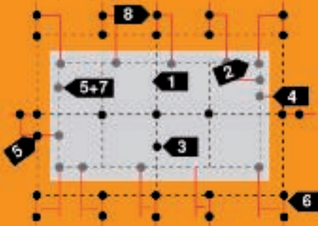
Functional equipotential bonding conductor and ring earther
